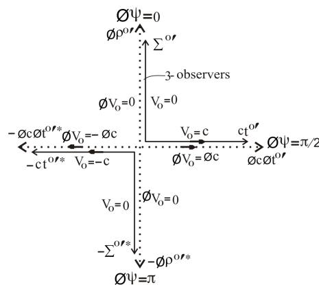
Fig. 8: b) The one-dimensional proper spaces \rho' and -\rho'^* in Fig. 6b transform into proper time dimensions c\tau^{0'} and -c\tau^{0'*} respectively and the proper intrinsic spaces \phi\phi' and -\phi\phi'^* in Fig. 6b transform into proper intrinsic time dimensions \phi c\phi t^{0'} and -\phi c\phi t^{0'*} respectively relative to 3-observers in the proper Euclidean 3-spaces \Sigma^{0'} and -\Sigma^{0'*} (represented by lines) along the vertical.
