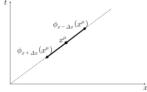
Fig. 3: Two contributions to \phi(x) .
