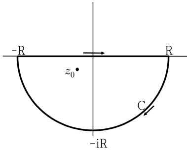
Fig. 4: Contour of integration.
