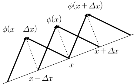
Fig. 2: Contributions to each \phi .
