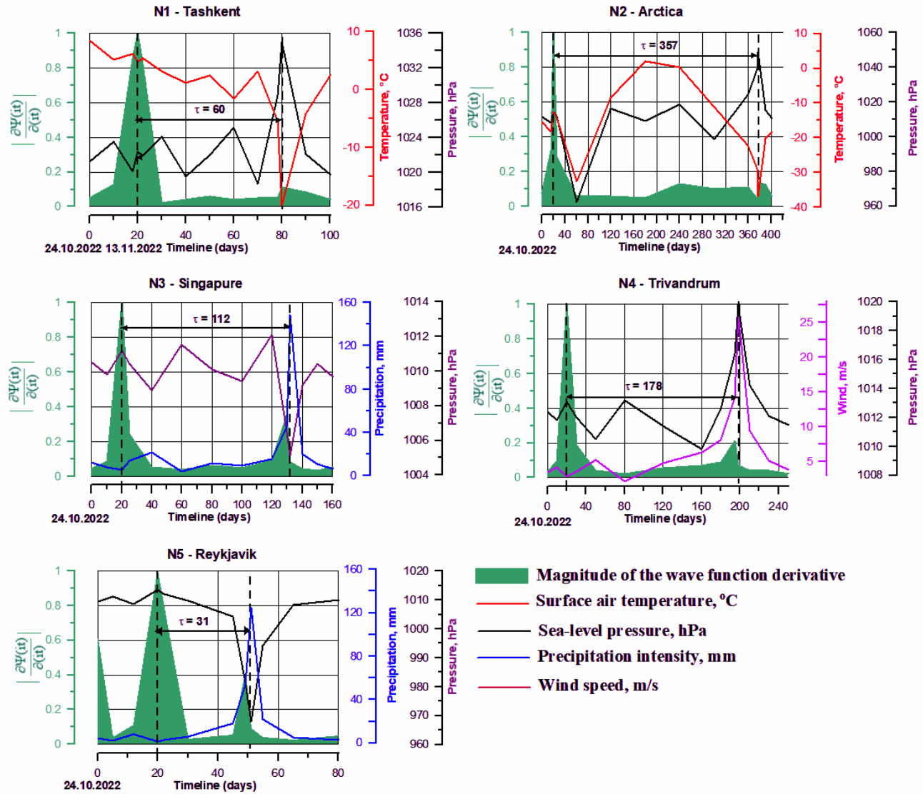
Fig. 1: Results of numerical modeling of the phase relationship between atmospheric and biophysical parameters based on the comprehensive prognostic equation (1) for five global nodes (2022–2023).
